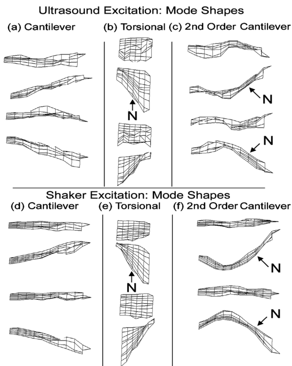
FIG. 4. Scanning vibrometer measurements of the displacement of the reed from its equilibrium position. Successive images downwards show displacement after 90^\circ phase shifts during the cycle; the N in the figures illustrates the location of the nodal line for the torsional and second-transverse modes. (a) and (d) are the first transverse mode of the cantilever at 726 Hz; (b) and (e) are the first torsional mode at 2.95 kHz, and (c) and (f) are the second transverse mode of the cantilever at 4.54 kHz. The deflection shapes of (a)–(c), using ultrasound stimulated excitation, were nearly identical to (d)–(f) that were obtained using a mechanical shaker.
